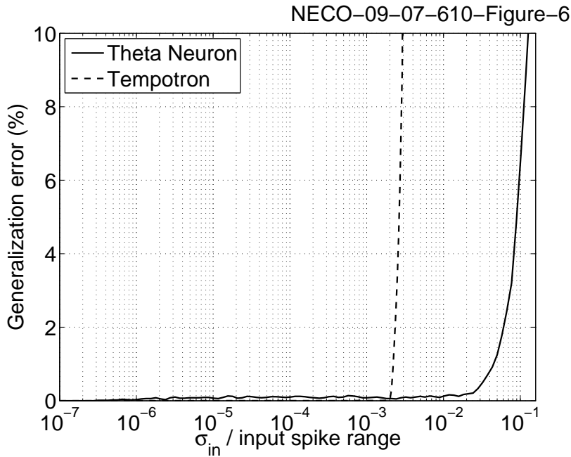
Figure 6: Jitter Comparison to Tempotron. A single neuron is trained with the method proposed here and by the method in (Gütig & Sompolinsky, 2006). The number of synapses and input patterns is 500 ( \alpha = 1 ). I_o = -0.005 and w_{ini} = 0.01 . For the theta neuron, training is stopped when classification error becomes zero. The theta neuron is shown to be much less sensitive to higher levels of jitter indicating better generalizability than the Tempotron. There is one pattern near the decision boundary (because classification error has just reached 0%) that is especially sensitive to low levels of jitter. In fact, this one pattern is the only one that gets misclassified until the normalized jitter reaches about 7 \cdot 10^{-3} . Training the network 7% longer after 0% classification error has been reached delays the first appearance of an error from a normalized jitter of 3.5 \cdot 10^{-7} to 1 \cdot 10^{-3} .
