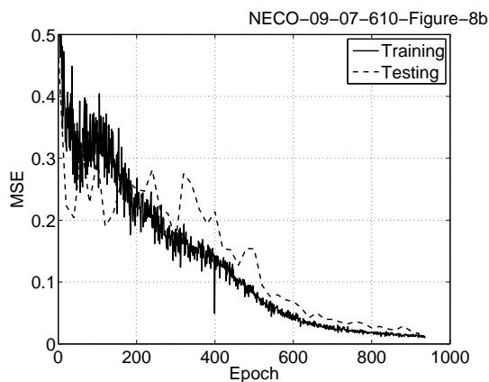
(b) Sexton 5 MSE Results. Testing data was generated every 10 epochs.
