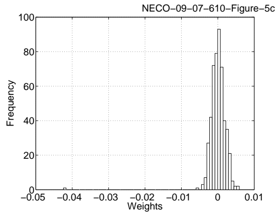
(c) Learned Weight Distribution. The weights form a normal distribution around zero with a slight skew towards positive weights. The slight positive skew ensures that output spikes will not be canceled. The single outlier is the weight associated with the reference input. As the number of inputs increases, the magnitude of the learned weights decreases as each input spike needs to effect the output spike time less and less.
