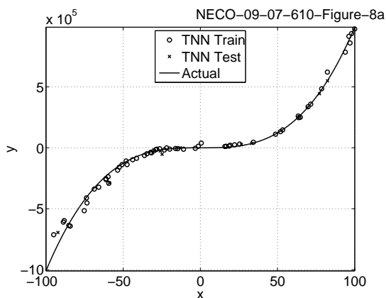
(a) Sexton 5 Regression Results. Both the testing and training patterns are in high agreement with the Sexton 5 function.
