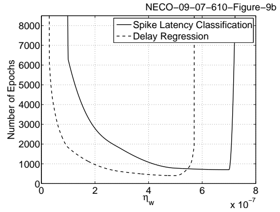
(b) Learning Rate ( \eta_w ) vs. Training Time. The optimal \eta_w for this set of parameters is 5e-7 for the delay regression data set and 7e-7 for the spike latency pattern data set.
