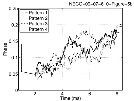
(b) Area of Phase Modulation. The period of time during which input spikes arrive is shown. The reference spike occurs at 1 ms. Class 1 patterns spend more time above the above the positive fixed point, while class 2 patterns spend more time below the positive fixed point thus causing them to produce later output spikes as desired.
