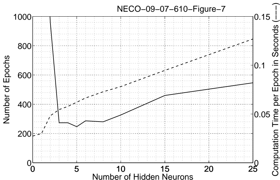
Figure 7: Hidden Neuron Analysis. This plot shows the effects of varying the number of hidden neurons, N , on the XOR problem. The dataset is trained to 0% classification error with \eta_w=1e-6 , I_o=-0.005 and w_{ini}=0.01 . As N increases, the computation time per epoch (the actual CPU time taken to perform the necessary calculations) also increases as expected since the number of parameters is increasing. The number of epochs needed for training has a minimum at N = 5 , where there are neither too many nor not enough trainable parameters to perform the XOR computation.
