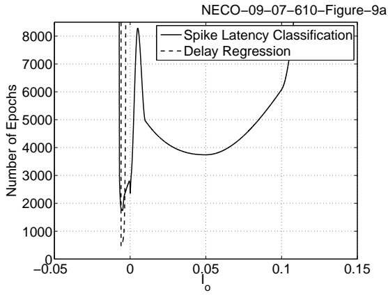
(a) Baseline Current ( I_o ) vs. Training Time. The optimal I_o for this set of parameters is -0.006 for the delay regression data set and -0.005 for the spike latency pattern data set.
