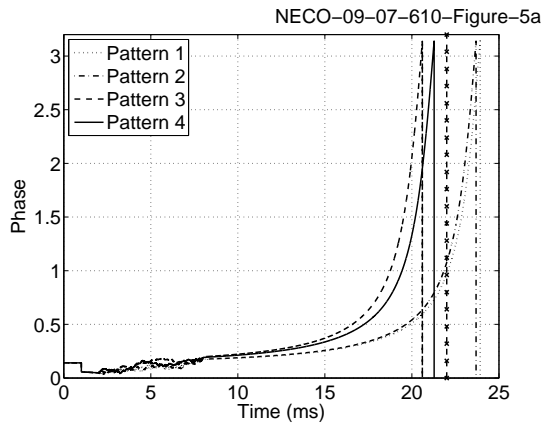
(a) Complete Phase Plot. The output spikes for all patterns shown fall on the desired side of the class decision line (the vertical line marked with 'x').
