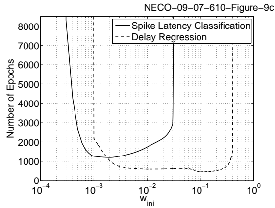
(c) Initial Weight ( w_{ini} ) vs. Training Time. The optimal w_{ini} for this set of parameters is 0.1 for the delay regression data set and 0.002 for the spike latency pattern data set.
